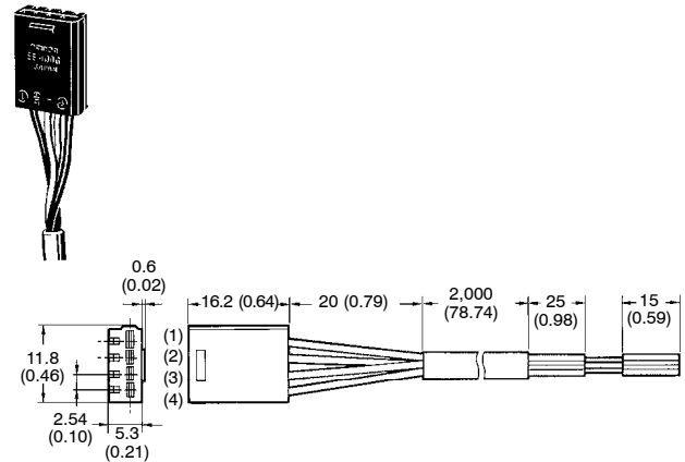
Terminal Arrangement
